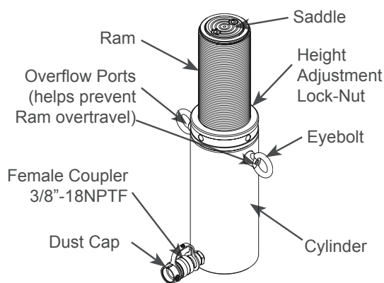
Figure 1 - Typical Cylinder Components
