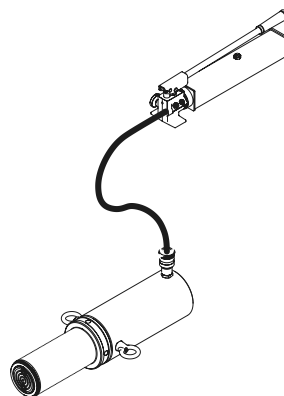
Figure 2 - Illustration to bleed air from system
