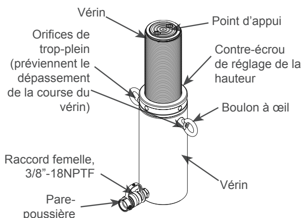
Figure 1 - Composants de vérin type
