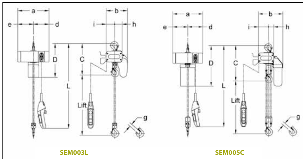
Model SEM005C
